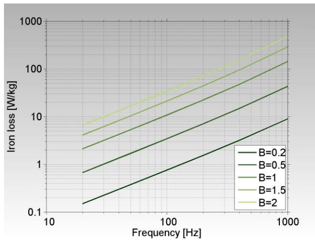
Figure 3: Iron loss as a function of frequency at different flux densities - at a mechanical density of 7.52 g/cm 3 .
