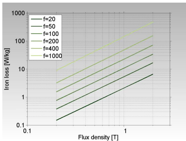
Figure 4: Iron loss as a function of flux density at different frequencies - at a mechanical density of 7.52 g/cm 3 .
