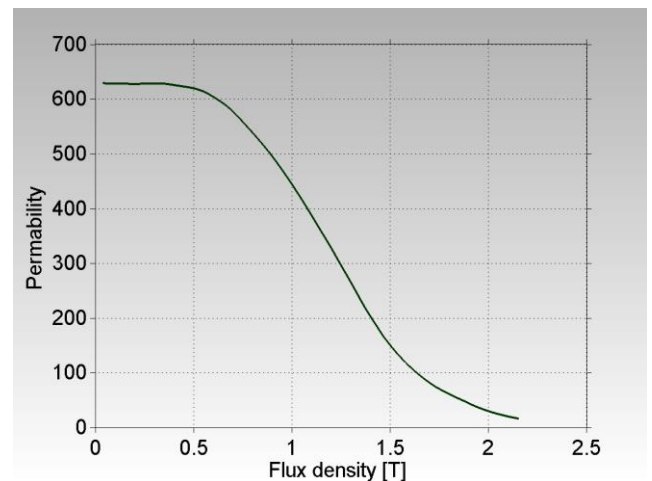
Figure 2: Permeability as a function of flux density for STX S7B SMC - at a mechanical density of 7.52 g/cm 3 .
