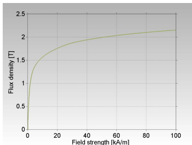
Figure 1: B-H curve for STX S7B SMC - at a mechanical density of 7.52 g/cm 3 .
