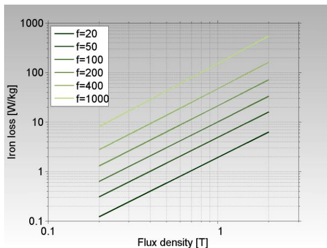
Figure 4: Iron loss as a function of flux density at different frequencies - at a mechanical density of 7.56 g/cm 3 .
