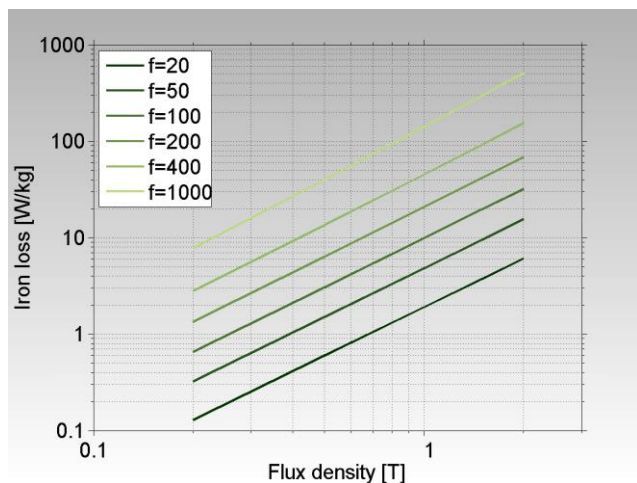
Figure 4: Iron loss as a function of flux density at different frequencies – at a mechanical density of 7.39 g/cm 3 .
