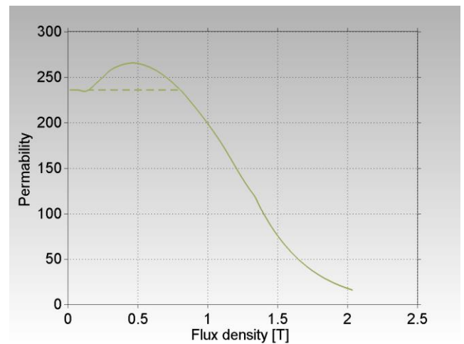
Figure 2: Permeability as a function of flux density for STX H1 SMC - at a mechanical density of 7.26 g/cm 3 .
