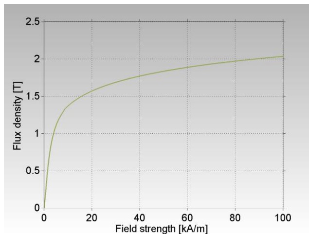
Figure 1: B-H curve for STX H1 SMC - at a mechanical density of 7.26 g/cm 3 .
