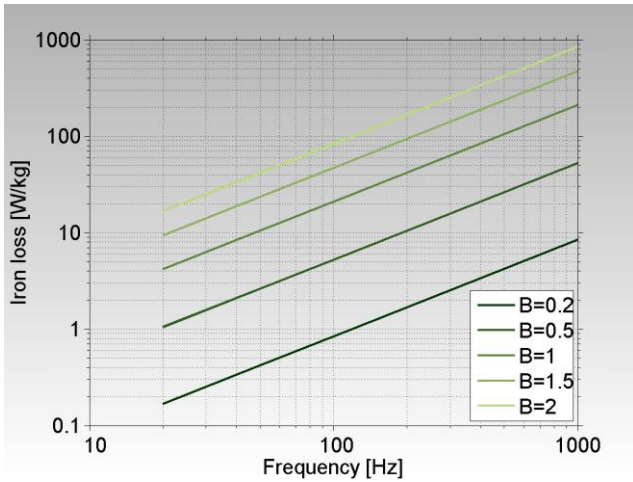
Figure 3: Iron loss as a function of frequency at different flux densities – at a mechanical density of 7.26 g/cm 3 .
