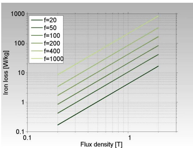
Figure 4: Iron loss as a function of flux density at different frequencies – at a mechanical density of 7.26 g/cm 3 .
