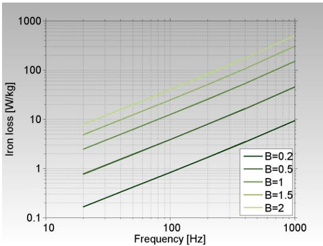
Figure 3: Iron loss as a function of frequency at different flux densities - at a mechanical density of 7.35 g/cm 3 .
