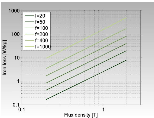
Figure 4: Iron loss as a function of flux density at different frequencies - at a mechanical density of 7.35 g/cm 3 .
