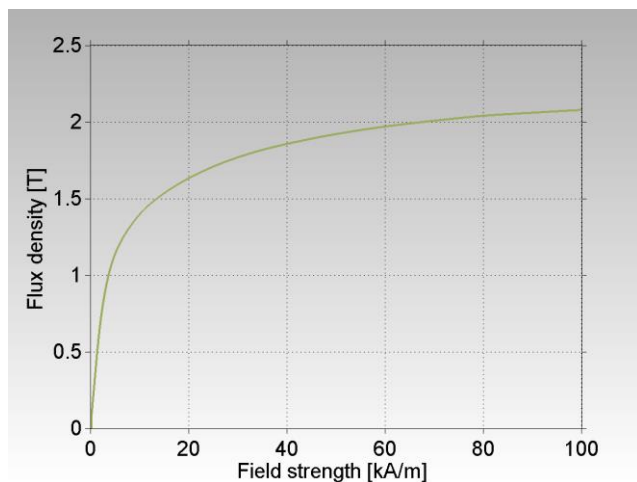
Figure 1: B-H curve for STX H 3 SMC - at a mechanical density of 7.35 g/cm 3 .
