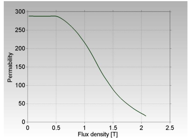
Figure 2: Permeability as a function of flux density for STX H 3 SMC - at a mechanical density of 7.35 g/cm 3 .
