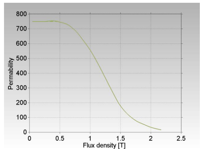
Figure 2: Permeability as a function of flux density for STX S7 SMC - at a mechanical density of 7.57 g/cm 3 .
