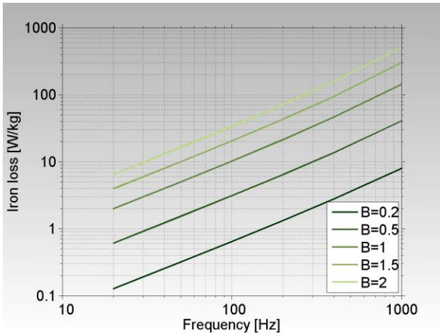
Figure 3: Iron loss as a function of frequency at different flux densities - at a mechanical density of 7.57 g/cm 3 .
