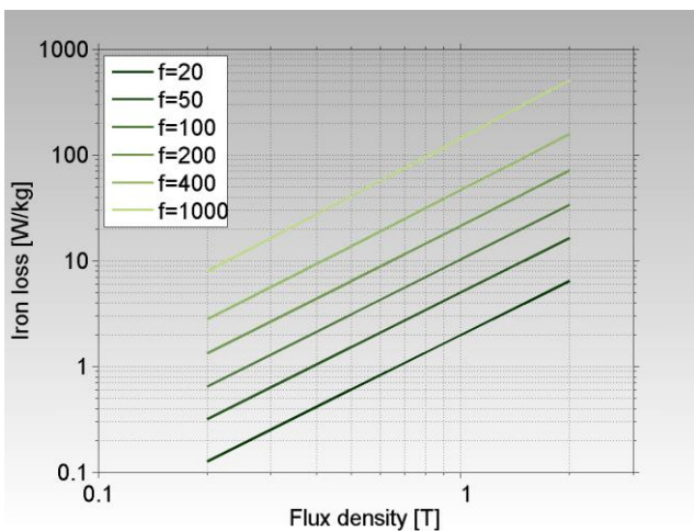
Figure 4: Iron loss as a function of flux density at different frequencies - at a mechanical density of 7.57 g/cm 3 .
