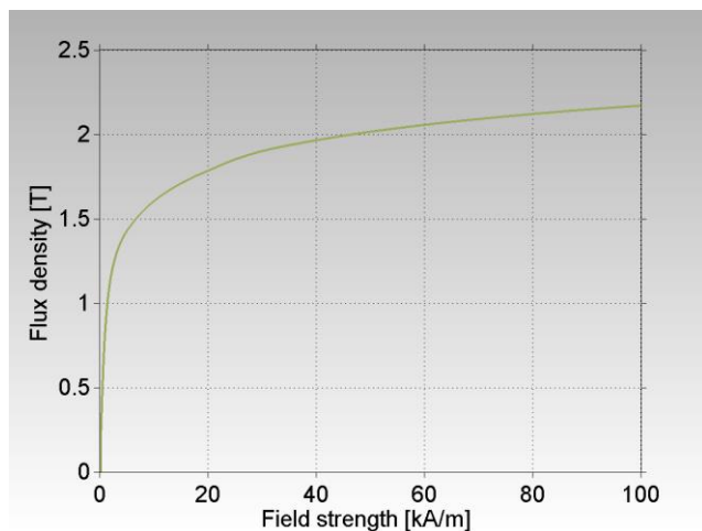
Figure 1: B-H curve for STX S7 SMC - at a mechanical density of 7.57 g/cm 3 .
