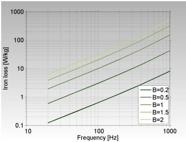
Figure 3: Iron loss as a function of frequency at different flux densities - at a mechanical density of 7.56 g/cm 3 .
