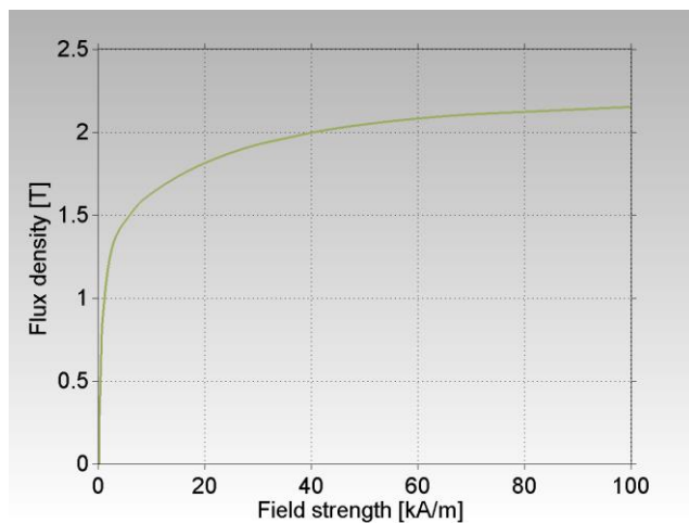
Figure 1: B-H curve for STX S10 SMC - at a mechanical density of 7.56 g/cm 3 .
