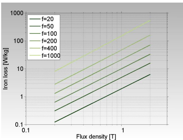
Figure 4: Iron loss as a function of flux density at different frequencies - at a mechanical density of 7.56 g/cm 3 .
