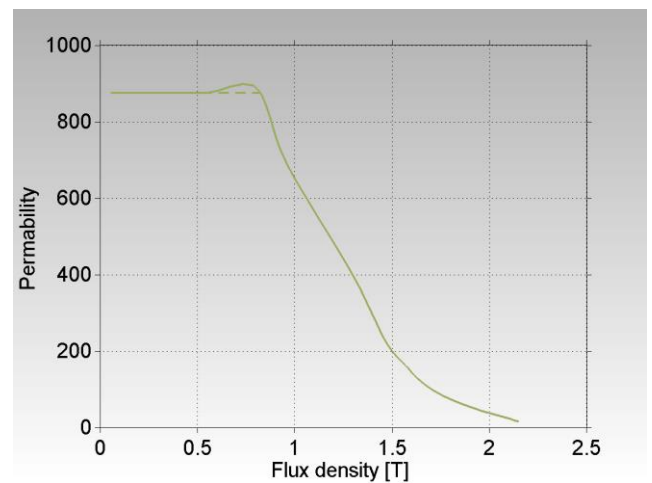
Figure 2: Permeability as a function of flux density for STX S10 SMC - at a mechanical density of 7.56 g/cm 3 .
