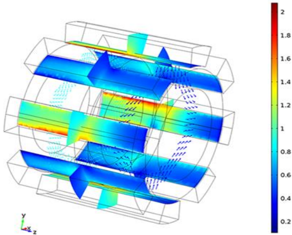
Figure 4: Finite element simulation of a magnetic gear
