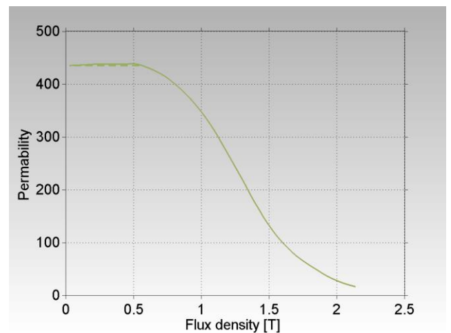
Figure 2: Permeability as a function of flux density for STX B7 SMC - at a mechanical density of 7.45 g/cm 3 .
