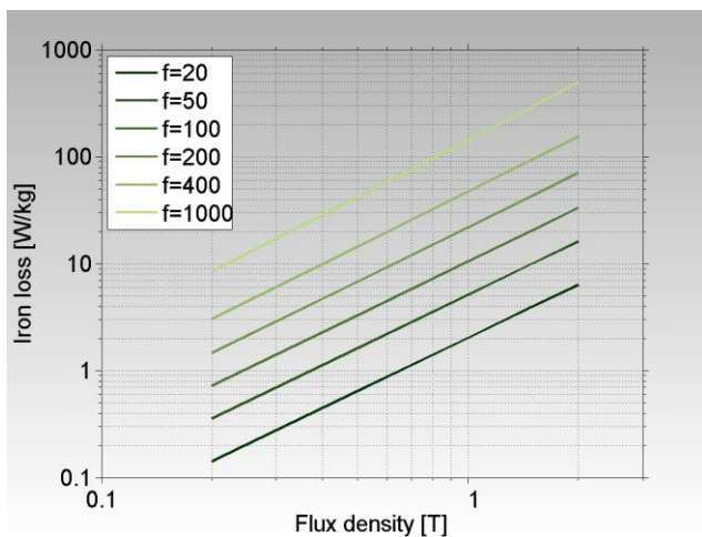
Figure 4: Iron loss as a function of flux density at different frequencies - at a mechanical density of 7.45 g/cm 3 .
