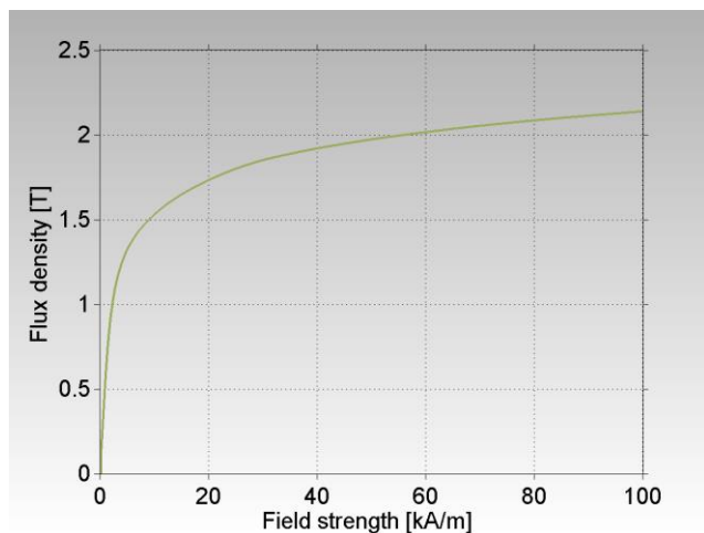
Figure 1: B-H curve for STX B7 SMC - at a mechanical density of 7.45 g/cm 3 .
