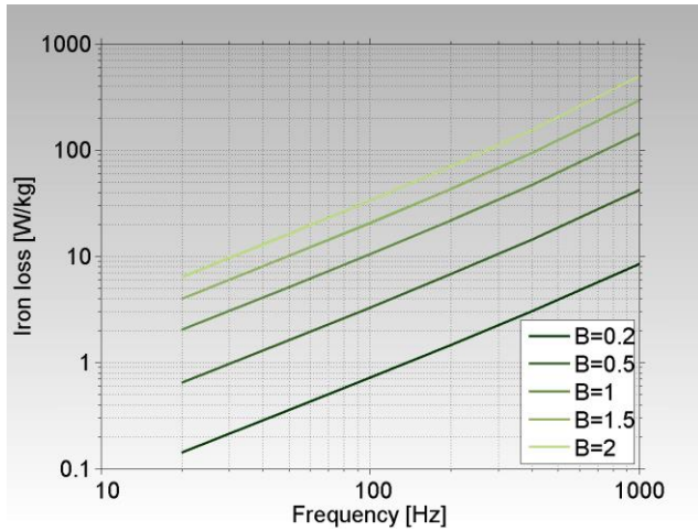
Figure 3: Iron loss as a function of frequency at different flux densities - at a mechanical density of 7.45 g/cm 3 .
